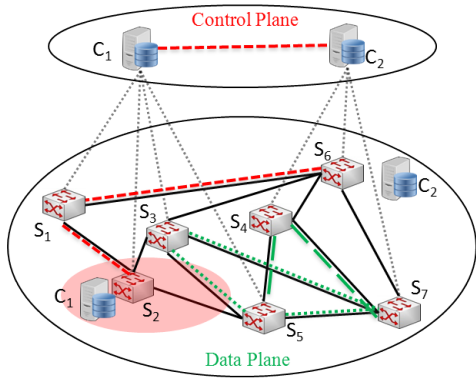
Fig. 3. After an alert is issued (red circle), switches served by the affected controller C_1 have to be assigned to their secondary controller (i.e., C_2 ). The virtual network embedded to switches S_7 - S_5 - S_3 have to be re-allocated as well, including the migration of a virtual node ( S_3 to S_4 ) and two virtual links ( (S_3, S_5) and (S_3, S_7) ).
